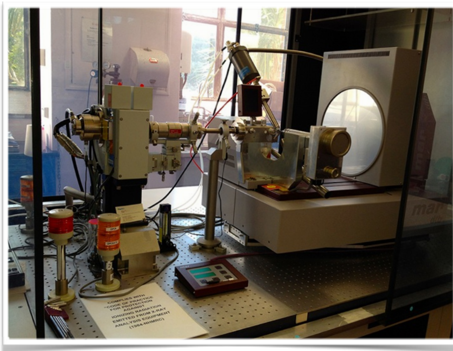
Rigaku MicroMax 007 HF rotating anode X-ray generator
